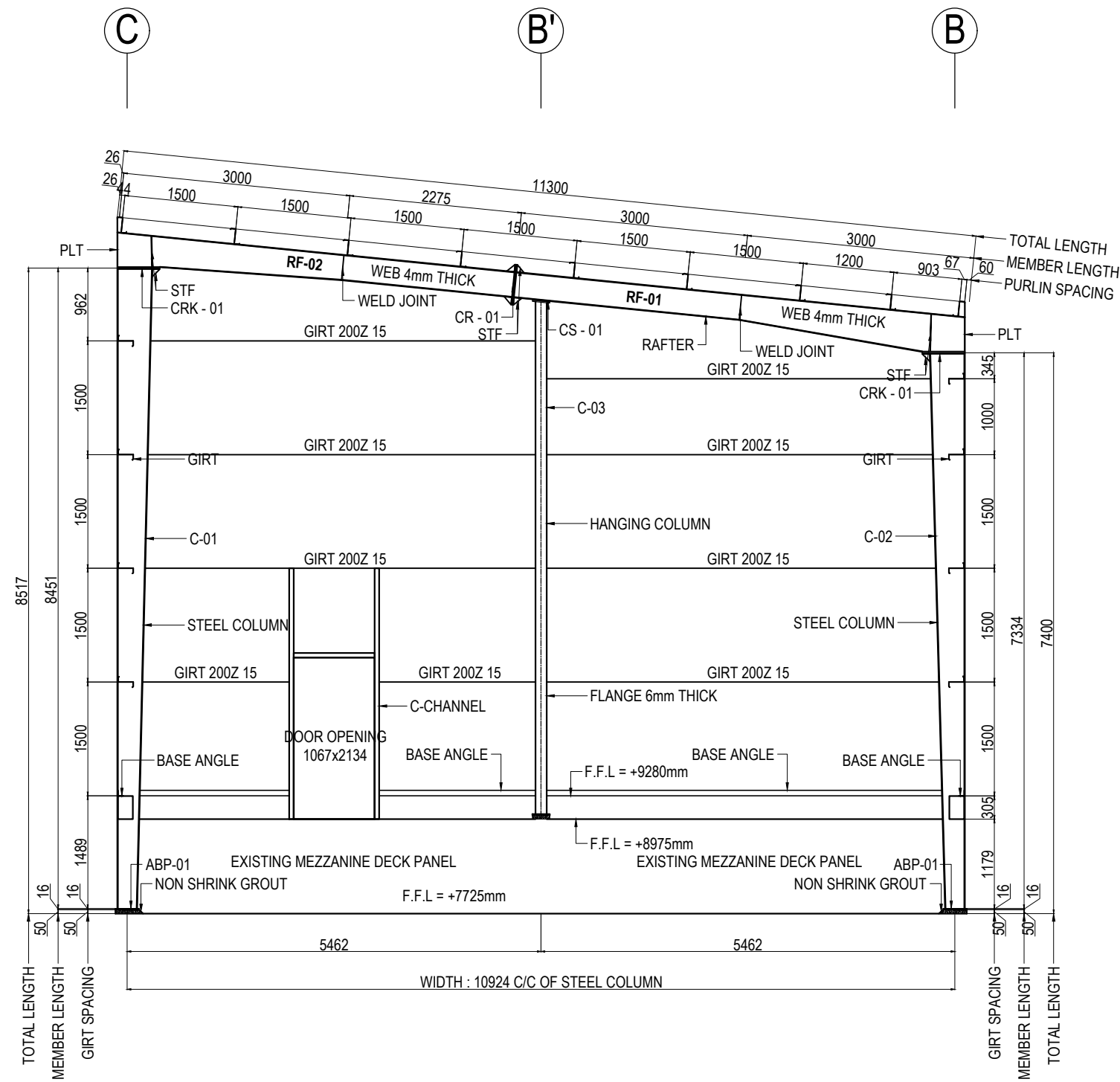
END WALL FRAMING @ GRID - 1
